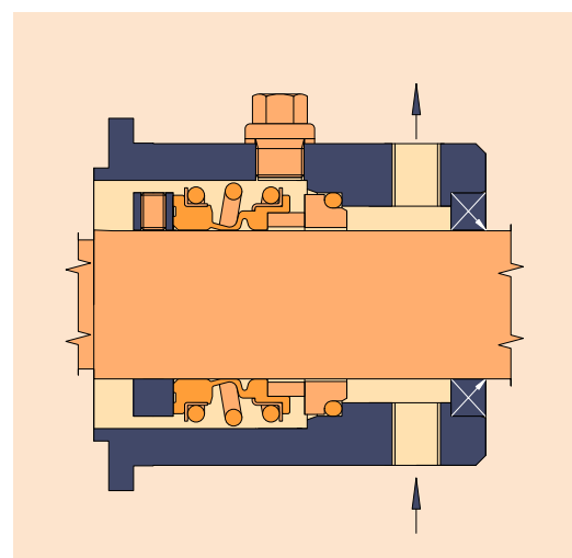
Fig. 4: Single mechanical seal + quench
