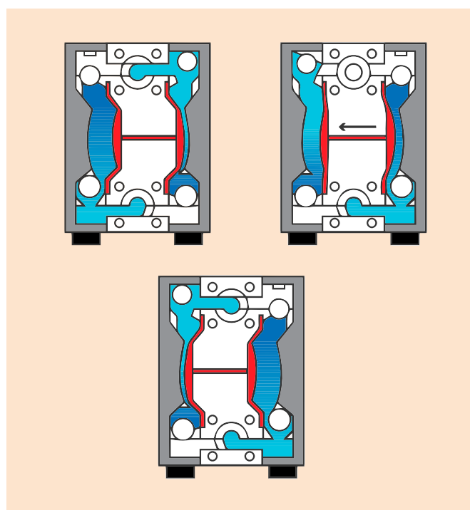
Fig. 9: Working principle of a double diaphragm pump
