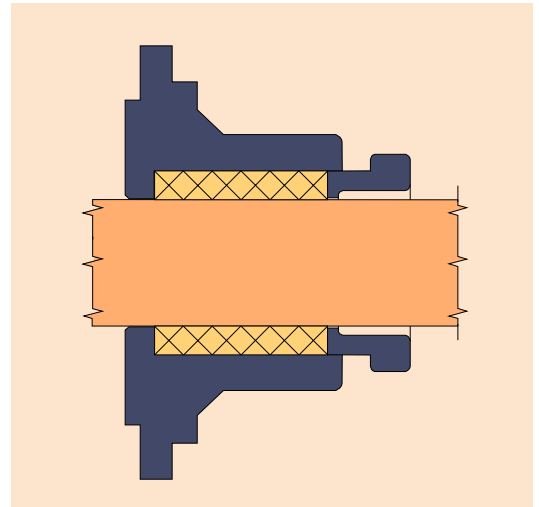
Fig. 1: Pumpshaft with packing gland containing 6 packing rings.
