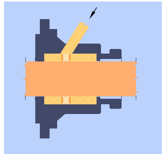
Fig. 2: Packing gland with 2 packing rings, lantern ring with quench and 3 packing rings
