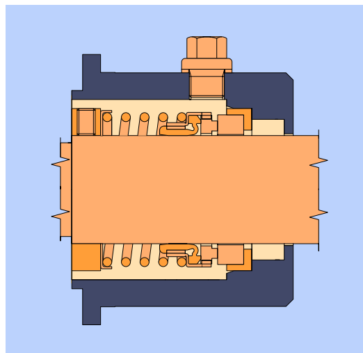
Fig. 3: Single mechanical seal
