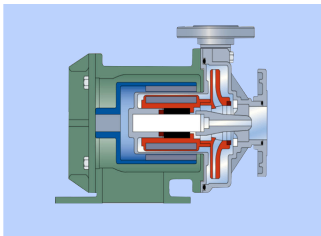
Fig. 6: Working principle of a magnetic driven centrifugal pump
