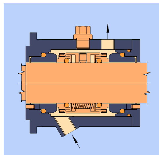
Fig. 5: Shaft equipped with double mechanical seal
